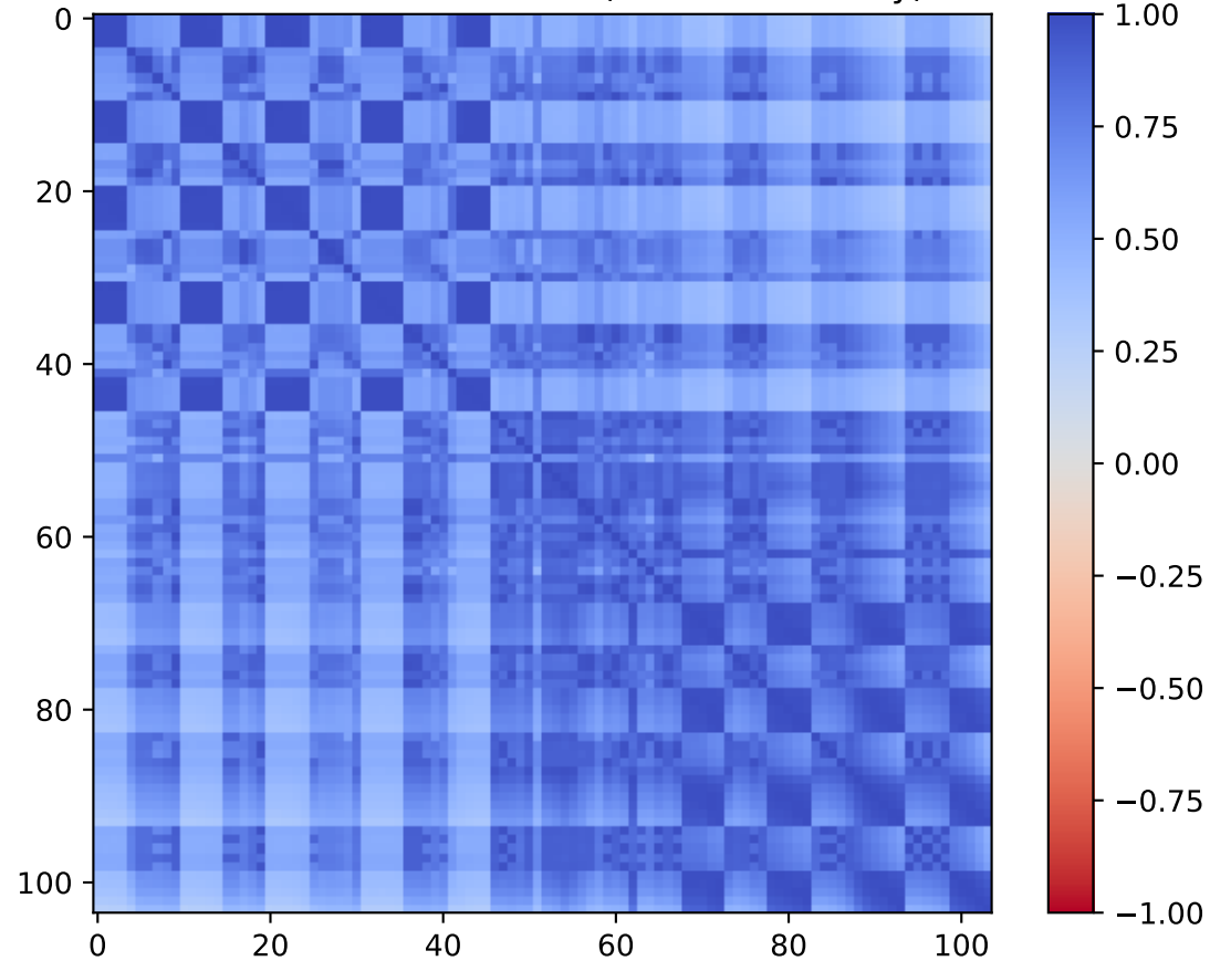
MC Gradient Covariance (Cosine Similarity)
